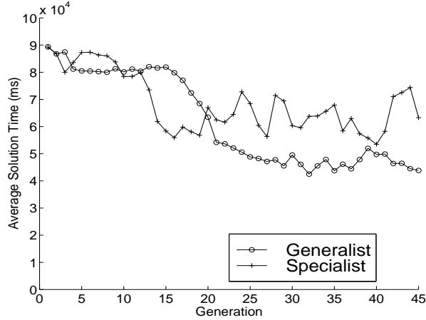
Figure 5: Comparison of average chromosome performance in generalist and specialist learning policies
