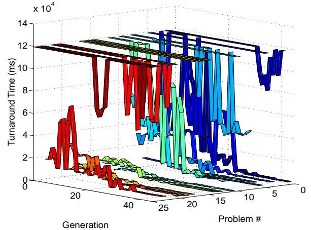
Figure 6: Turnaround time over 45 generations of the generalist learning policy
