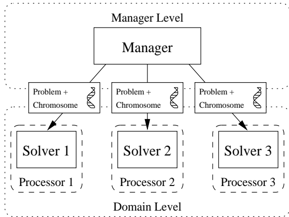
Figure 1: Two-level organization of problem-solving and learning tasks
