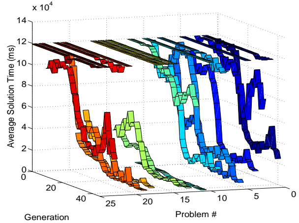
Figure 3: Average solution time over 45 generations of the generalist learning policy
