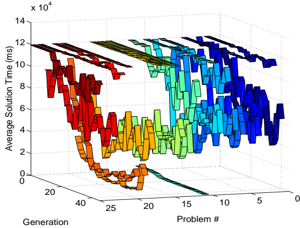
Figure 4: Average solution time over 45 generations of the specialist learning policy
