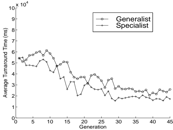
Figure 8: Comparison of turnaround time in generalist and specialist learning policies
