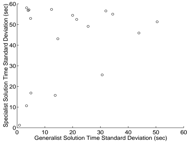
Figure 9: Comparison between standard deviation in solution times for specialist and generalist learning policies after 45 generations of learning
