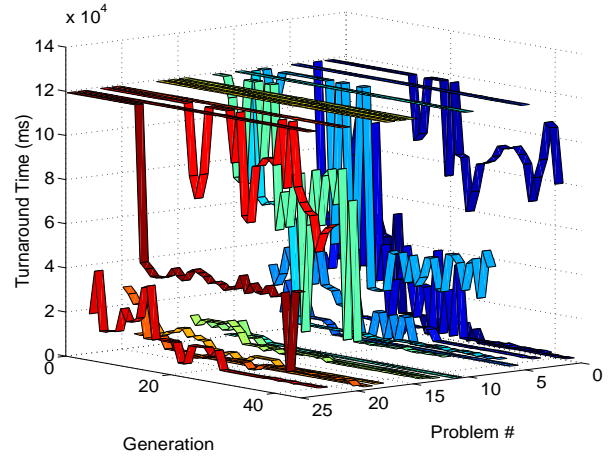
Figure 7: Turnaround time over 45 generations of the specialist learning policy
